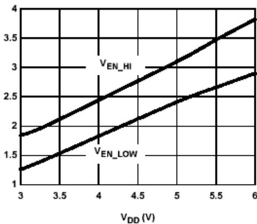
FIGURE 5. V_{EN\_HI} & V_{EN\_LOW} vs V_{DD}
